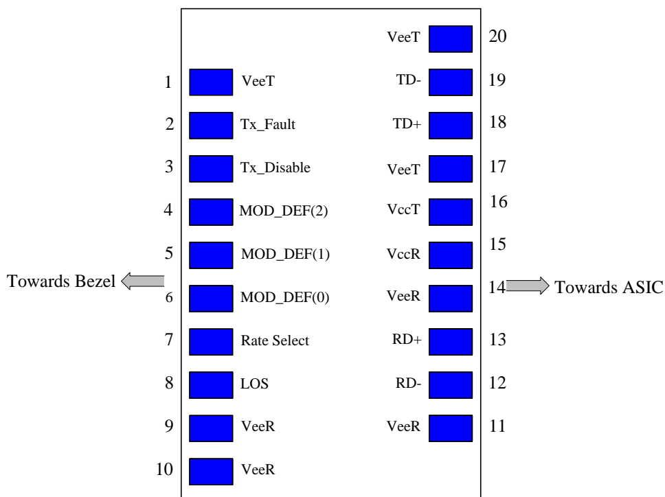
Figure 1 Transceiver pin descriptions
